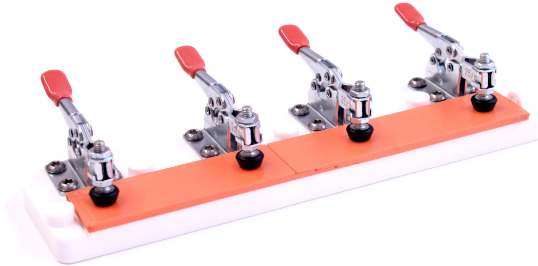
Fig. 5 – The fabricated fixture keeps a 3D-printed step-lap joint.
